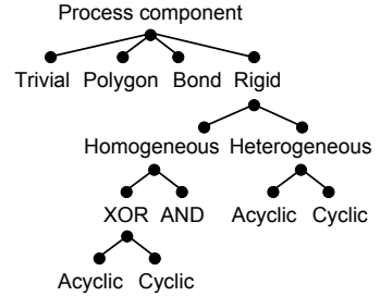
Fig. 2. Taxonomy
